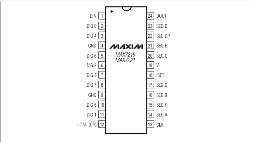
Figure 11-20. Pins on the MAX7221
