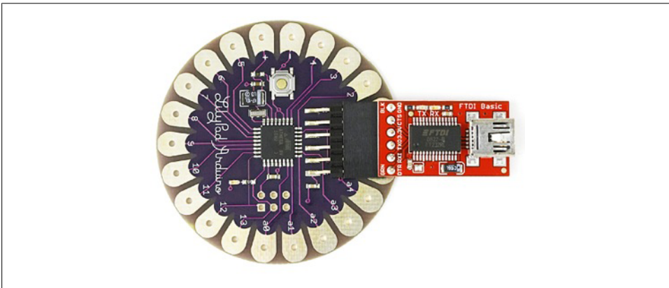
Figure 11-16. The LilyPad connected to a USB programmer
