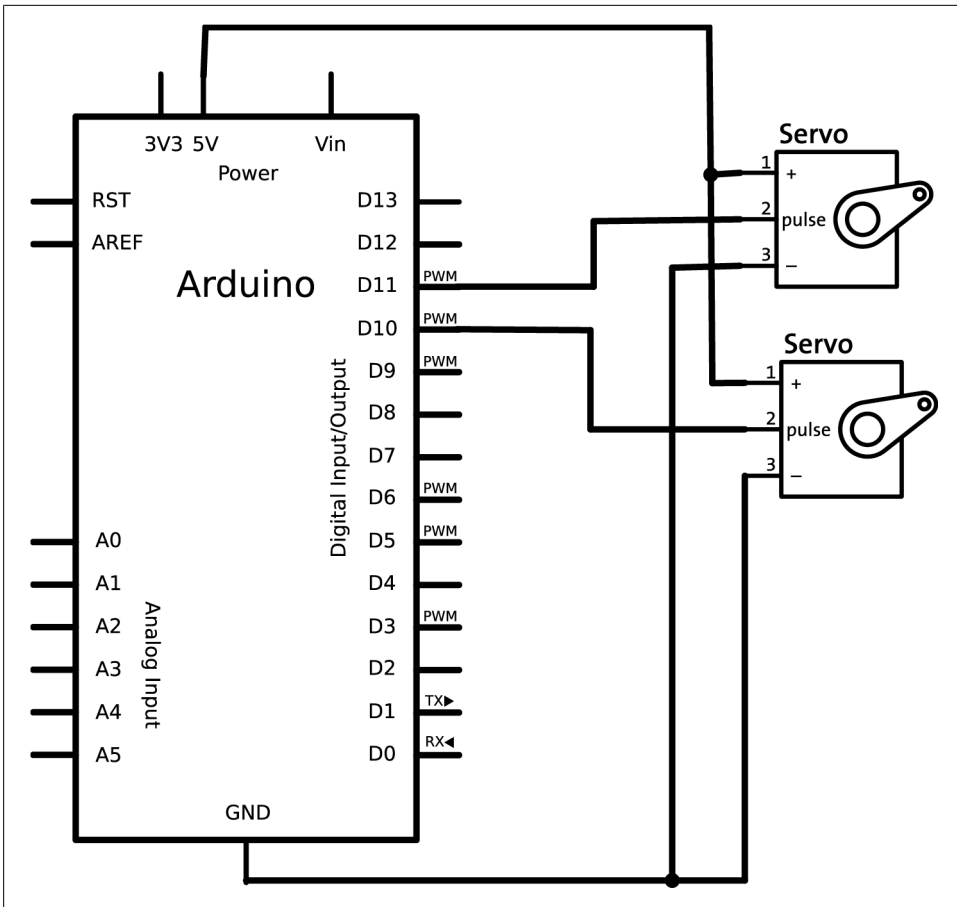
Figure 14-6. Connecting servos for face tracking
