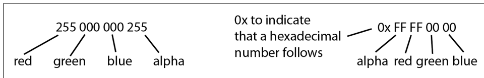
Figure 9-1. Numerical representations of pixel data
