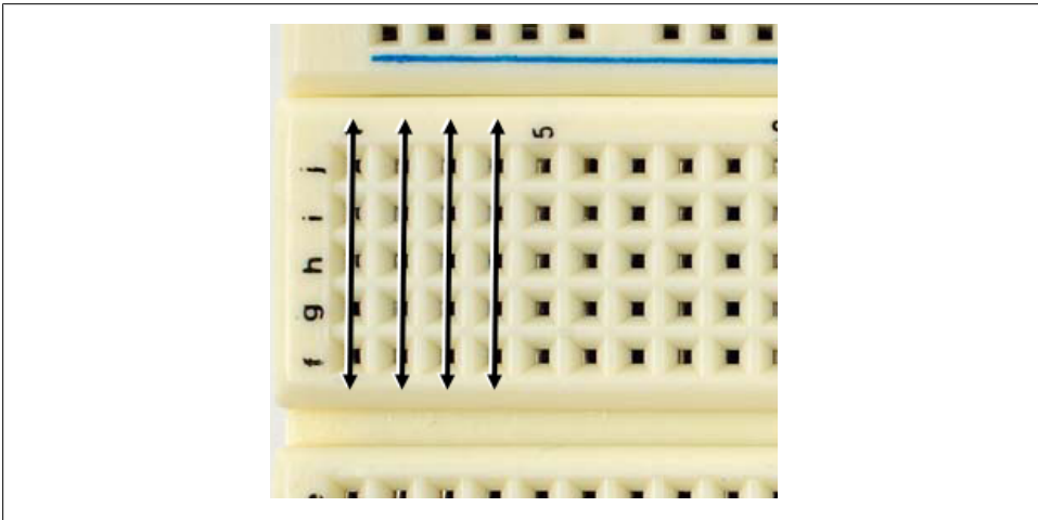
Figure 4-20. The middle of the board runs widthwise
