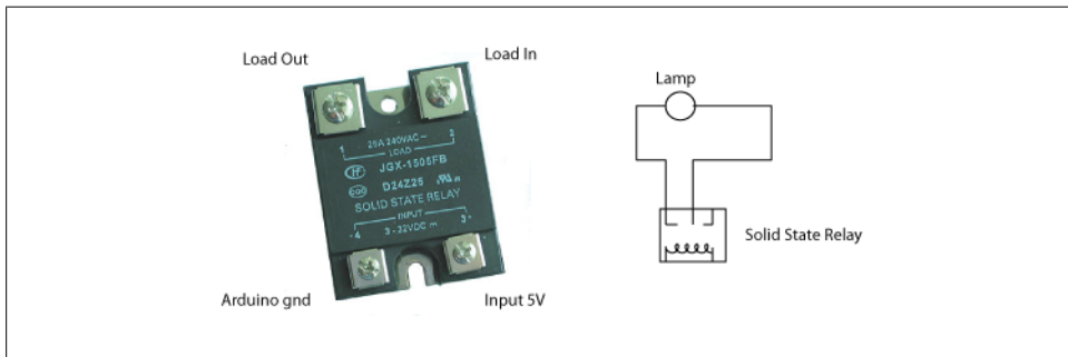
Figure 11-11. Using a solid-state relay with the Arduino controller
