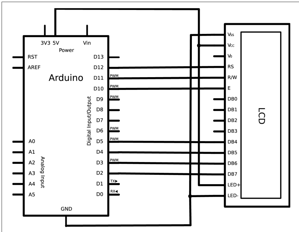
Figure 11-24. Connecting an LCD screen to the Arduino
