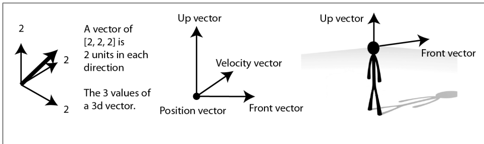
Figure 10-5. The vectors used by the FMOD Ex to place sounds and listeners
