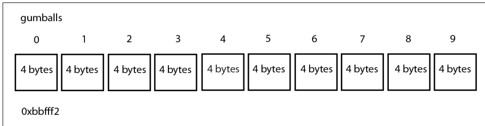
Figure 5-9. An array and a pointer
