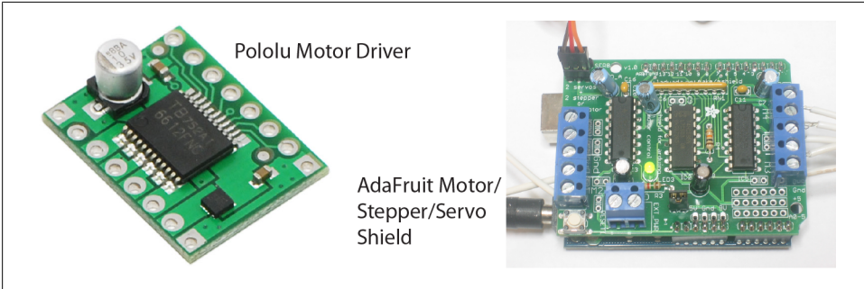
Figure 11-5. Two different motor driver shields
