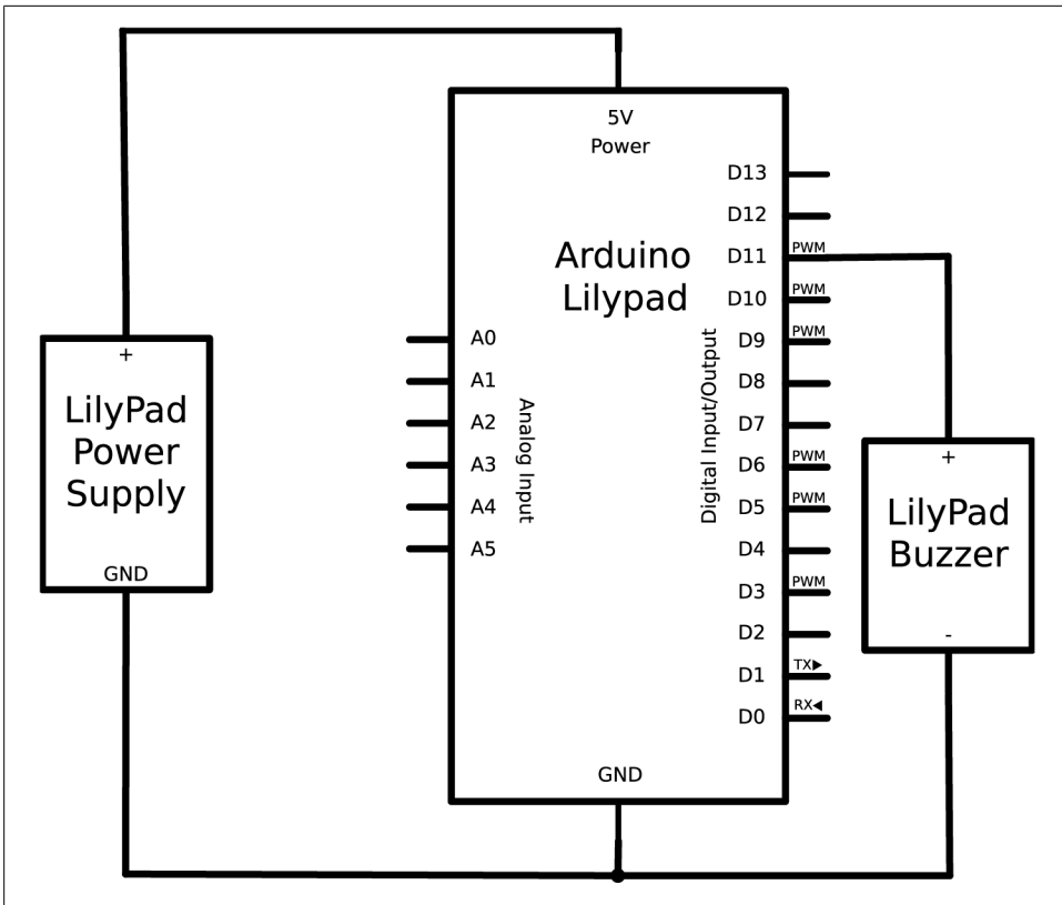
Figure 11-19. Connecting the Vibe Board
