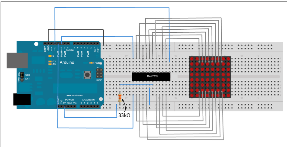
Figure 11-21. Connecting a 7221 to the Arduino shown here in breadboard view.
