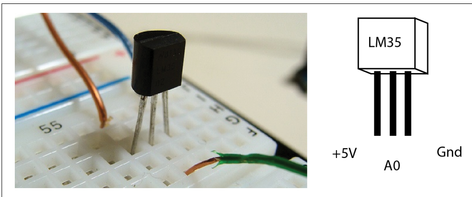
Figure 16-10. LM35 temperature sensor
