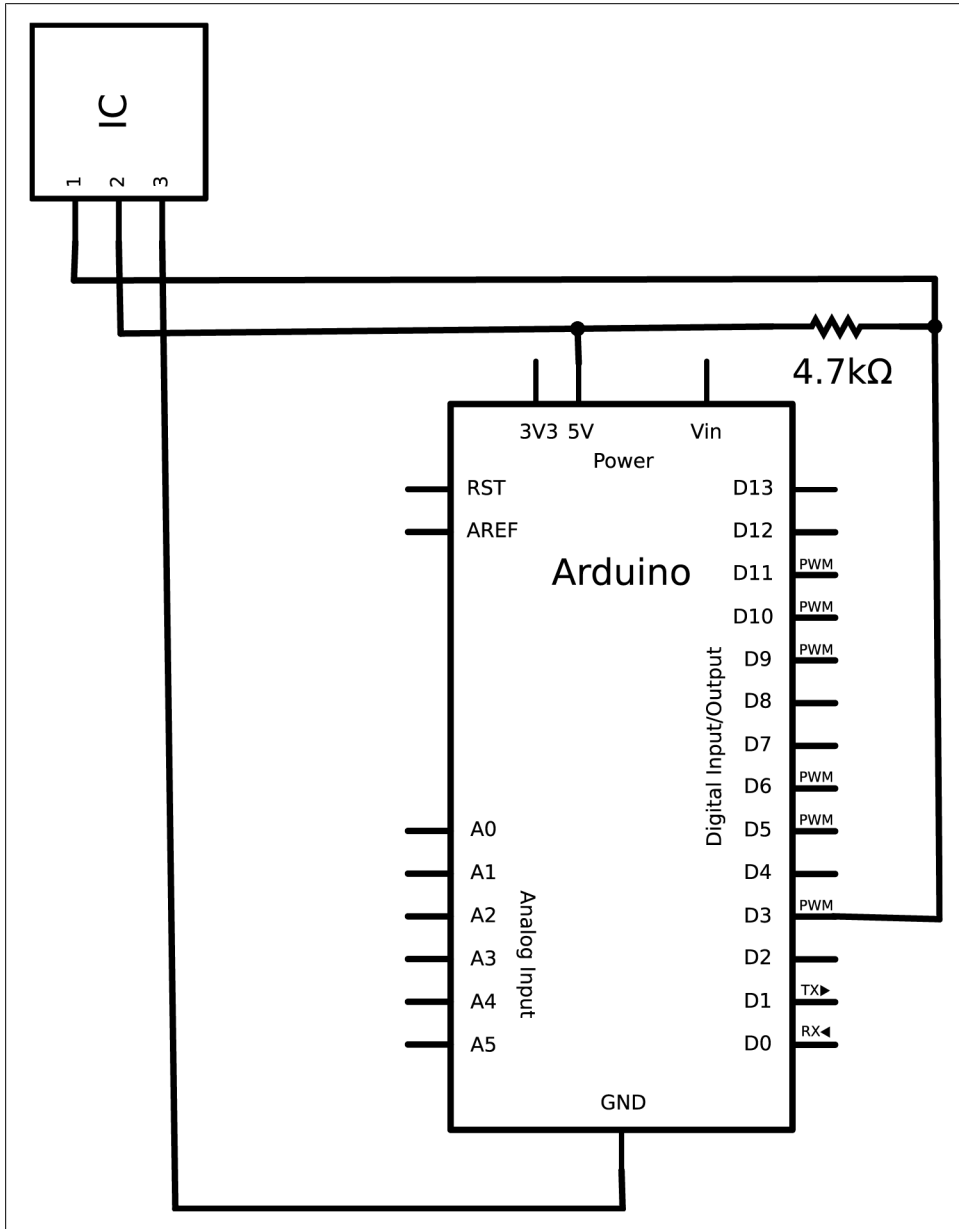
Figure 7-9. Connecting an PIR sensor to the Arduino board
