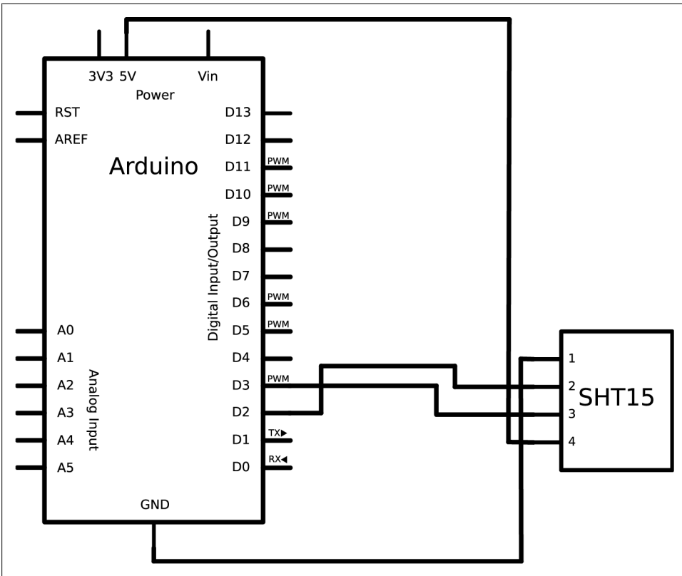
Figure 16-11. Connecting the SHT15 to the Arduino
