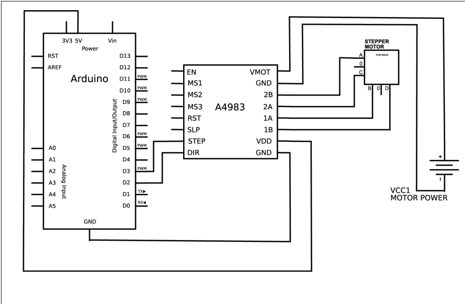
Figure 11-6. Connecting the Pololu Motor Driver to the Arduino
