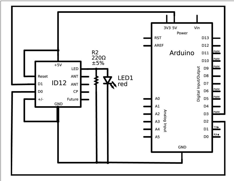
Figure 16-9. Connecting the ID-12 to the Arduino
