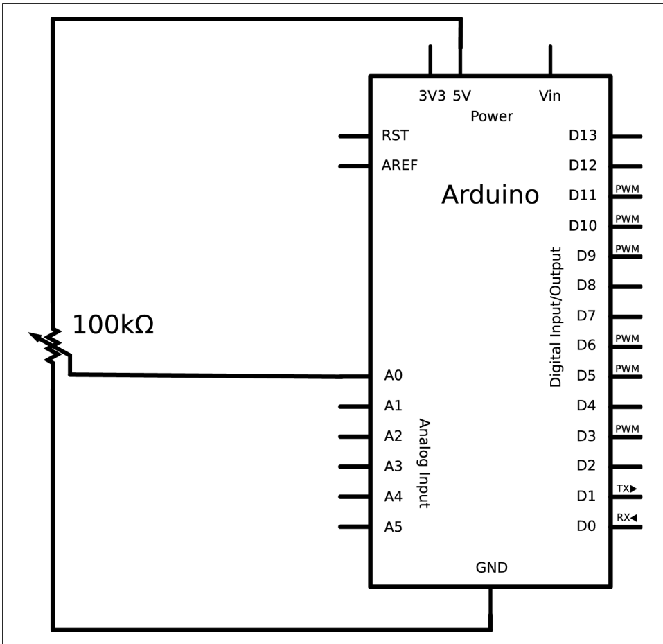
Figure 7-1. Connecting a potentiometer to an Arduino board
