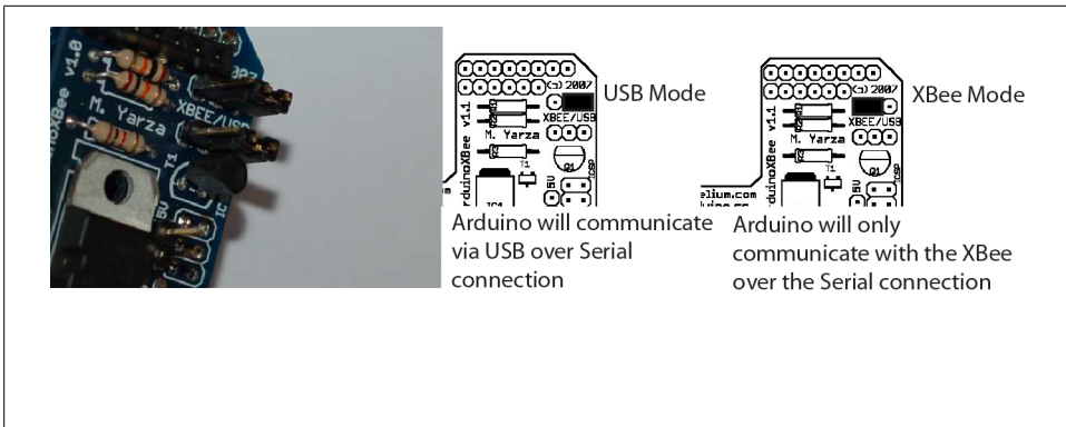
Figure 16-3. Jumpers on the XBee shield
