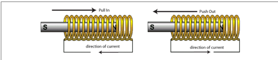
Figure 11-25. How a solenoid functions
