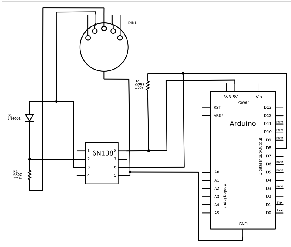
Figure 12-9. Wiring a MIDI-in connection
