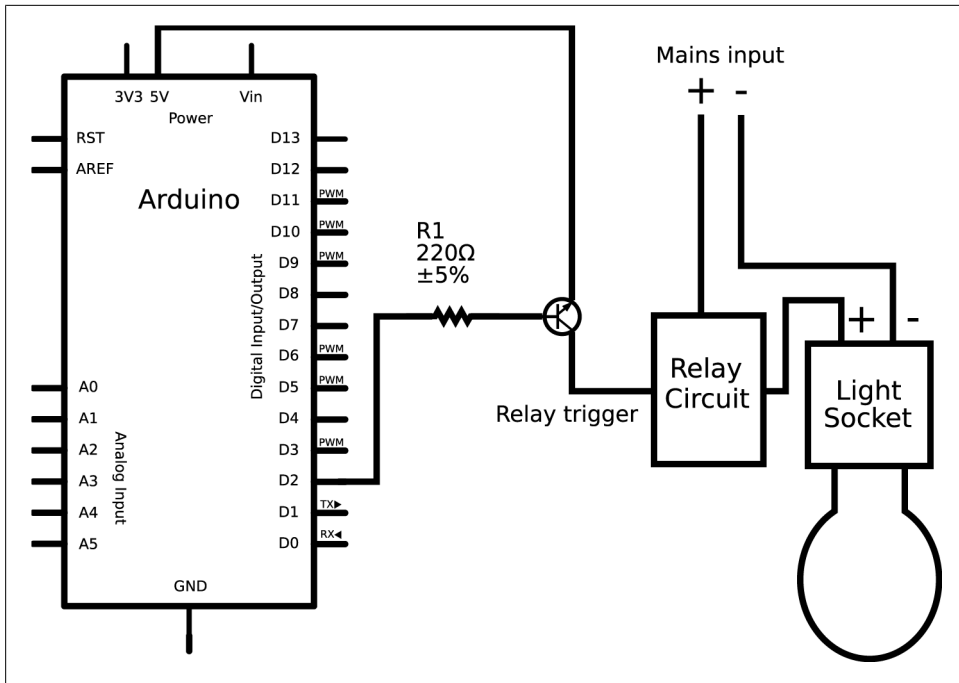
Figure 11-12. Connecting a lightbulb and a solid-state relay to the Arduino controller
