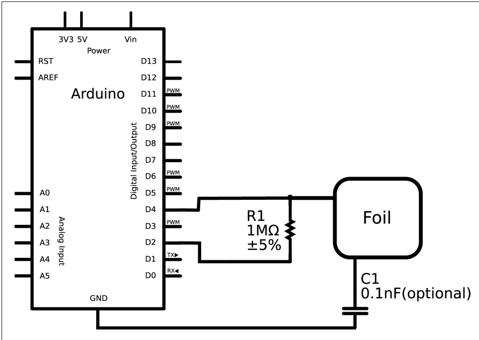
Figure 7-7. Using foil to sense changes in capacitance for the CapSense library
