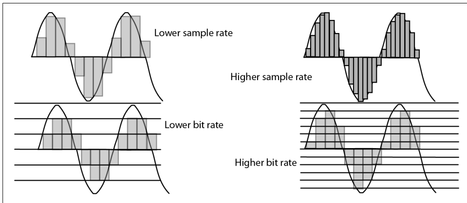
Figure 10-3. Sine wave representation of sound wave numeric values
