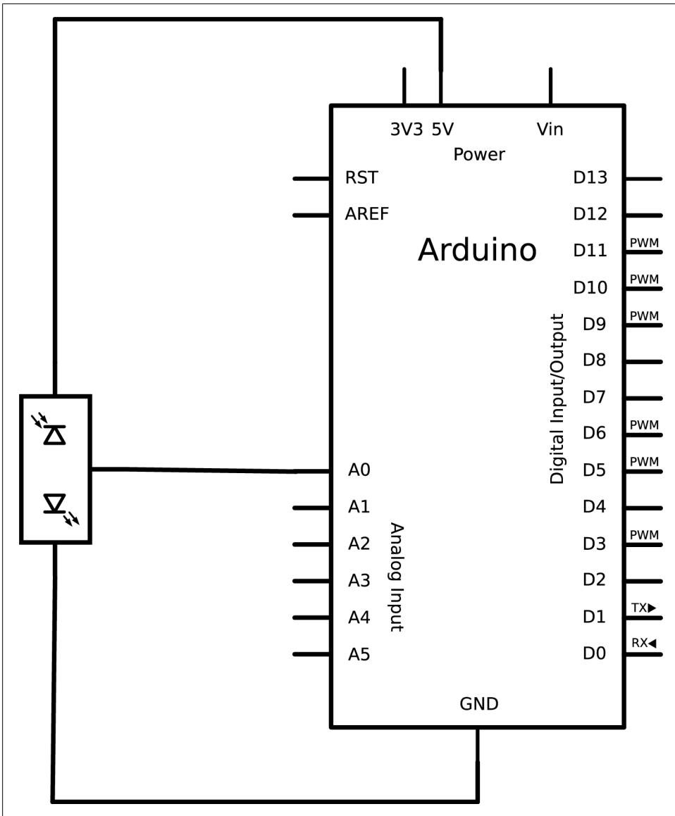
Figure 7-10. Connecting an infrared sensor to the Arduino board
