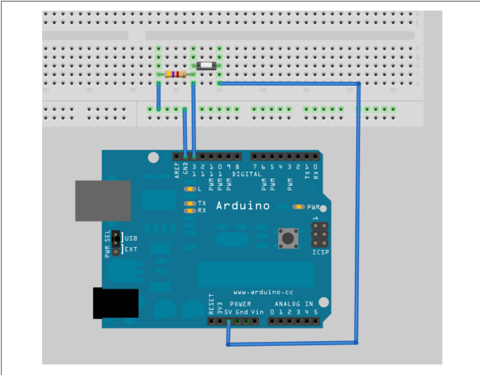
Figure 4-22. Wiring a button to the Uno
