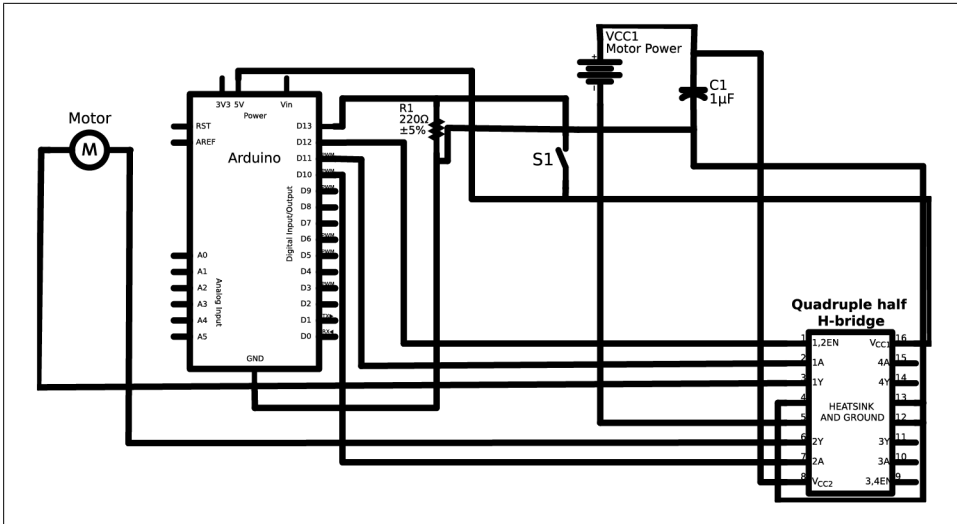
Figure 11-4. Wiring the motor and H-Bridge
