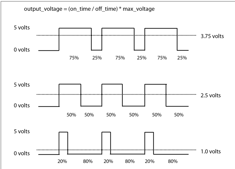
Figure 10-6. Pulse width modulation
