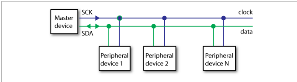
Figure 7-12. A controller using multiple devices over I2C
