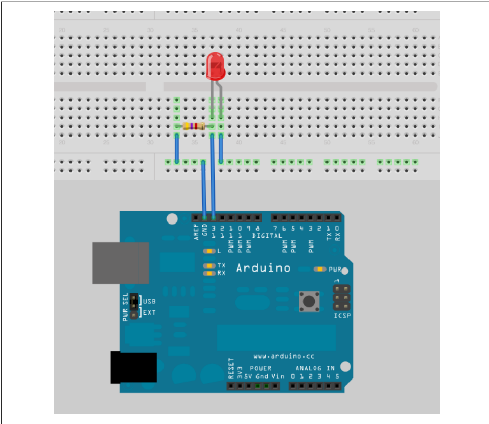
Figure 4-21. Uno with LED attached
