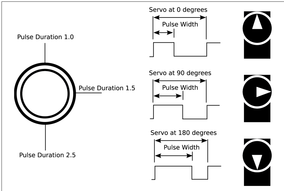
Figure 11-9. Positioning a servo using the pulse width or duration
