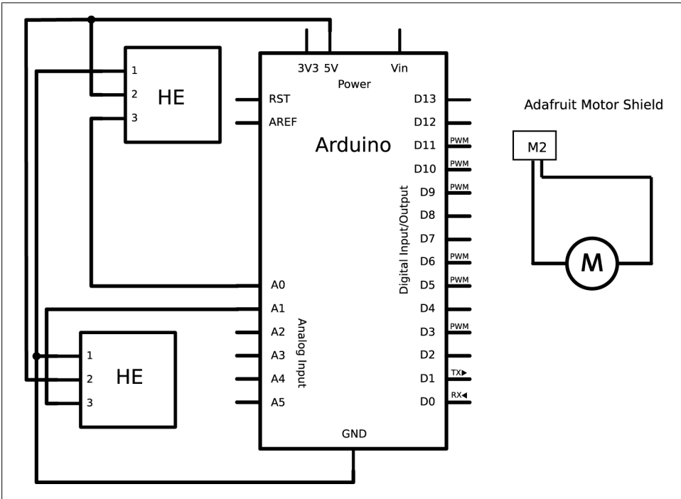
Figure 11-8. Connecting Hall effect sensors and a motor
