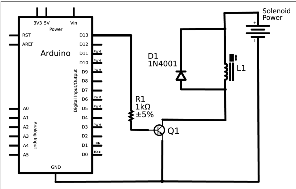
Figure 11-27. A circuit to connect a Solenoid (L1) to the Arduino
