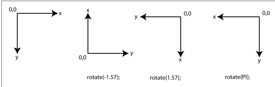
Figure 8-7. The rotate() method of the Processing language
