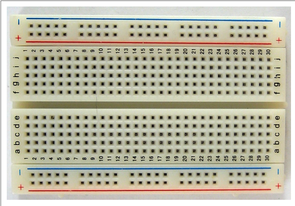
Figure 4-17. A breadboard or prototyping board
