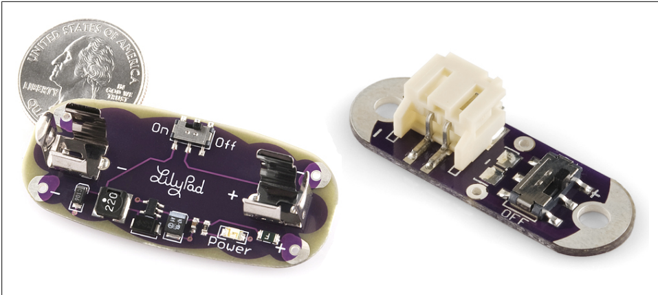
Figure 11-18. Lithium ion battery and the LiPower board
