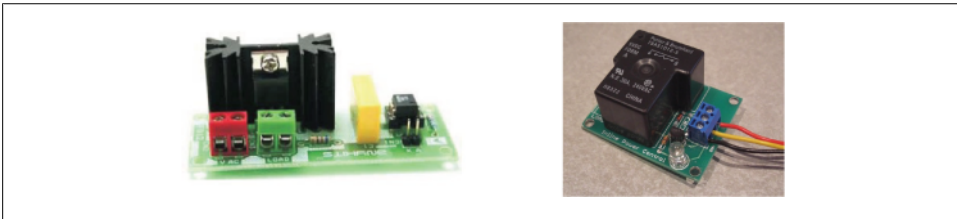
Figure 11-14. Two shields for working with household currents: the Anykits Solid State Relay Switch and the SparkFun Inline Power Control
