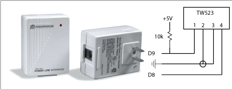
Figure 16-7. The TW523 X10 module
