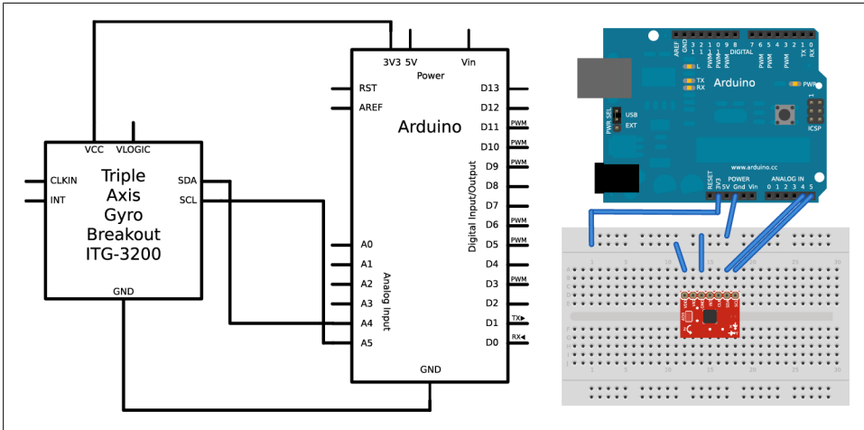
Figure 7-13. Connecting the ITG-3200 to the Arduino
