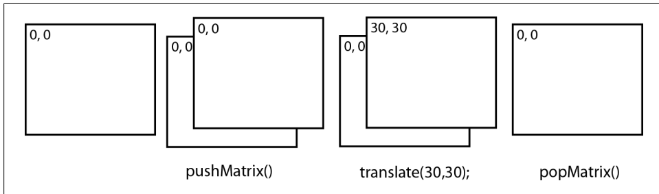
Figure 8-6. The coordinate matrix
