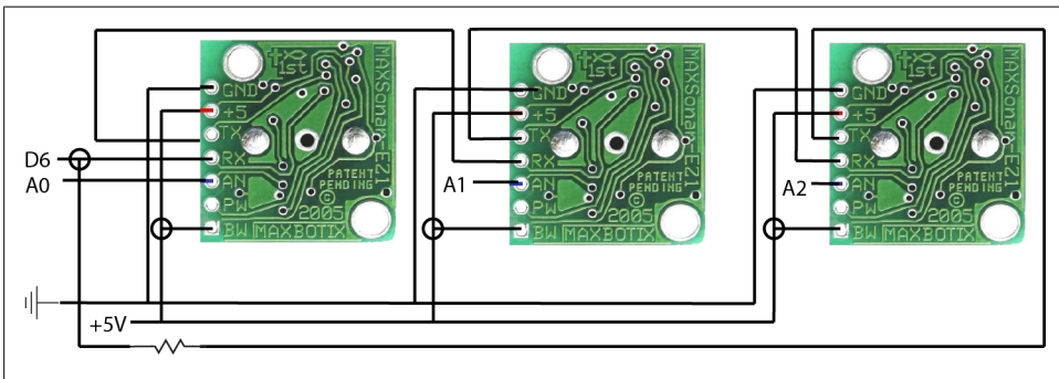
Figure 16-5. Daisy-chaining multiple ultrasonic sensors together
