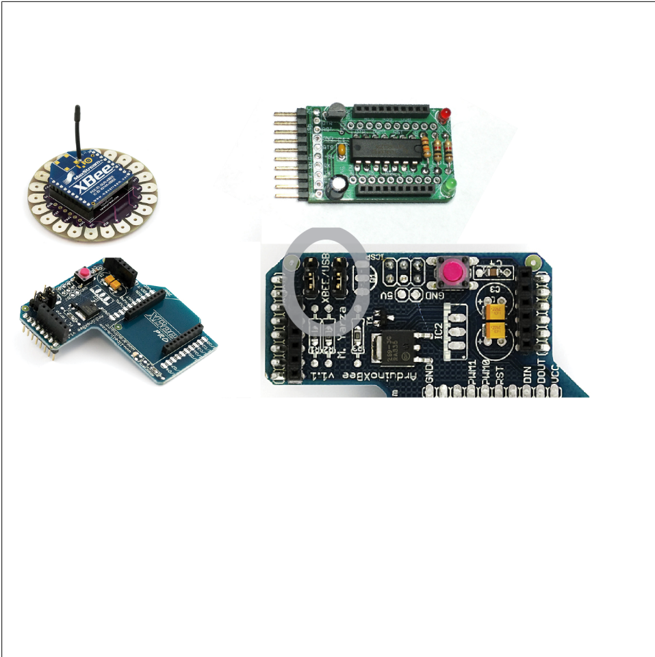
Figure 16-2. Clockwise from left: LilyPad XBee module, Adafruit XBee adapter, close-up of the jumper pins on the XBee Shield, the Arduino XBee shield
