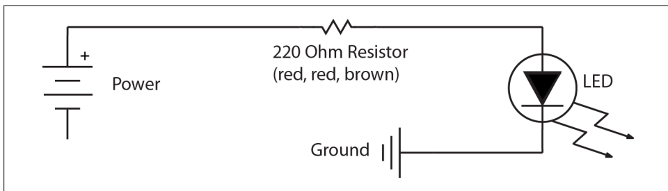
Figure 7-3. Connecting an LED
