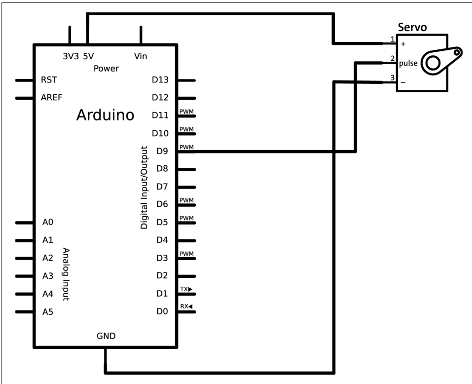
Figure 11-10. Connecting an Arduino to a servo motor
