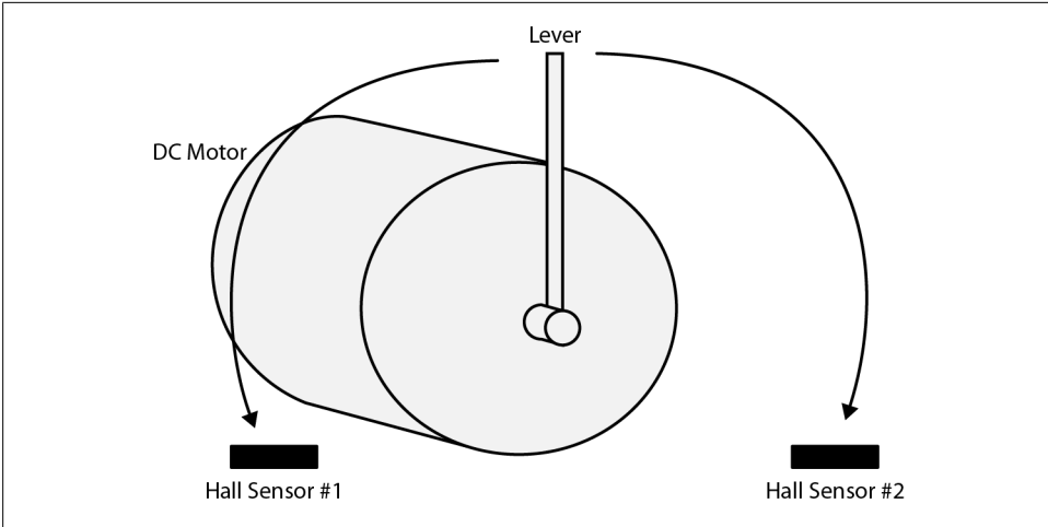
Figure 11-7. Using two Hall effect sensors for position estimation
