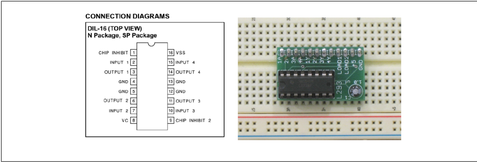
Figure 11-2. The pinout and image of the 1293 H-Bridge chip
