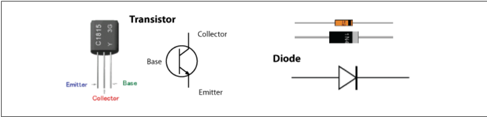
Figure 11-26. Transistors and diodes
