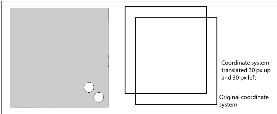
Figure 8-5. Transforming the coordinate space
