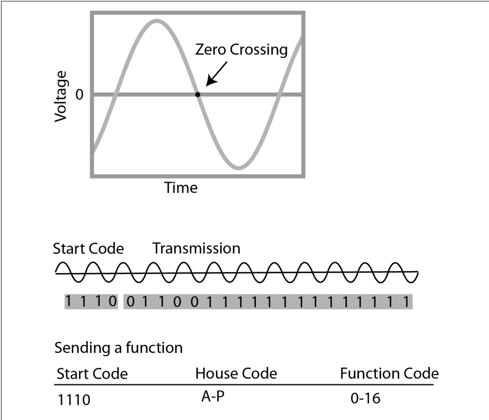
Figure 16-6. X10 sending data across the zero crossing of electrical current
