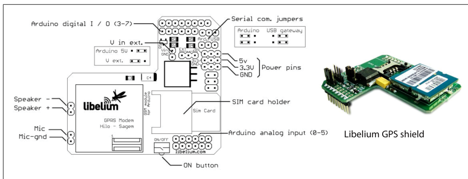
Figure 15-4. The Libelium GPRS shield and schematic
