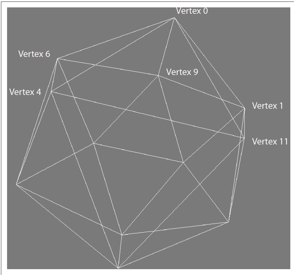
Figure 13-10. Each vertex is used multiple times to create each triangle of the icosahedron
