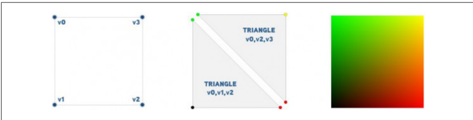
Figure 13-9. Creating a quad from two triangles
