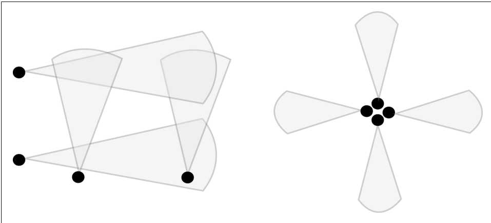
Figure 16-4. Two strategies for determining the location of an object using ultrasonic sensors
