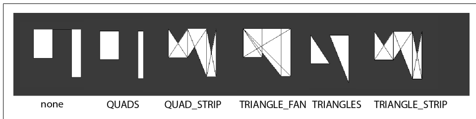
Figure 13-7. How different drawing modes handle the same set of vertices
