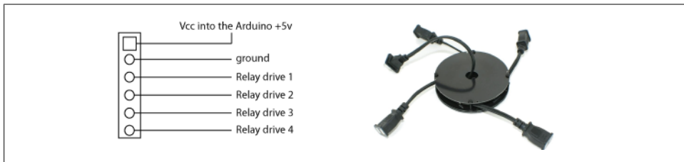
Figure 11-13. The pins on the RelaySquid
