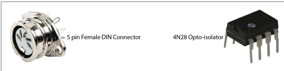
Figure 12-10. Components for creating Arduino MIDI in
