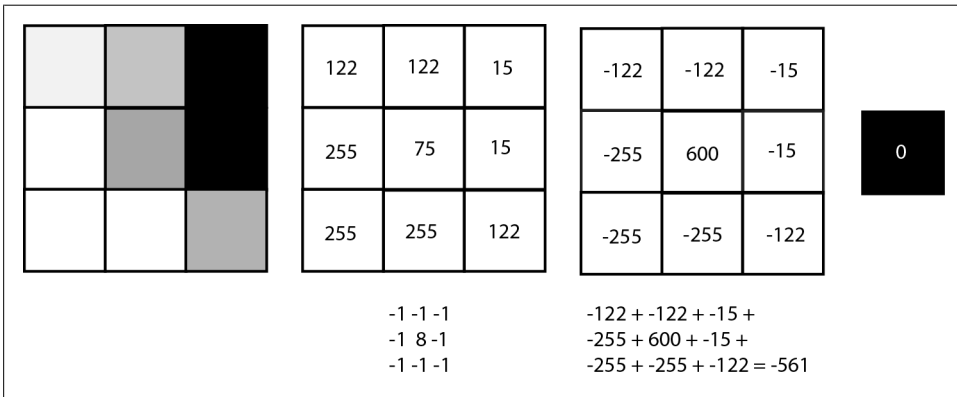
Figure 9-3. Performing an image convolution
