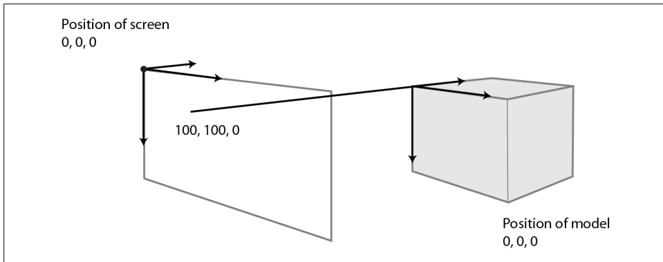
Figure 13-8. The model coordinate system and the screen coordinate system may not be the same values
