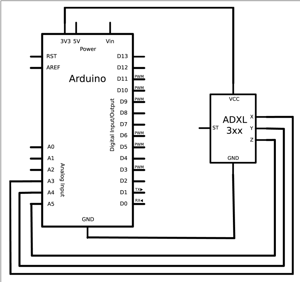
Figure 7-11. Connecting an accelerometer to the Arduino controller
