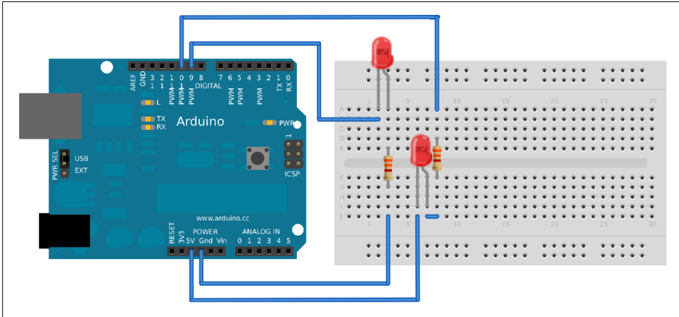
Figure 7-4. Wiring multiple LEDs to an Arduino board (all breadboard and schematic diagrams created with Fritzing.org)
